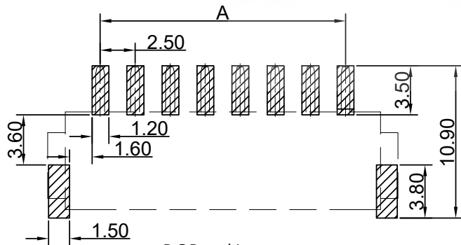
P.C.Board Layout General Tolerance: ±0.05
