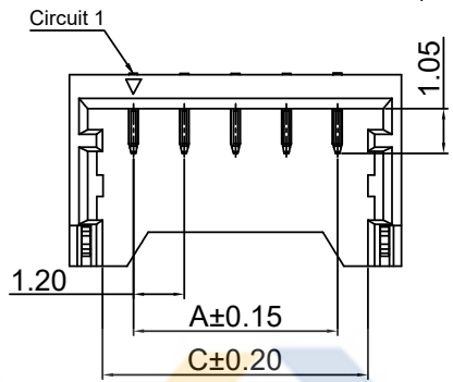
4~5 Pin Without Sticking Point
