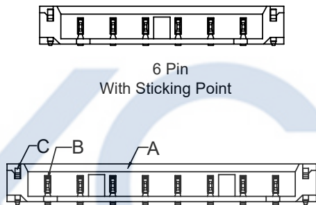
7~10 Pin With Sticking Point
