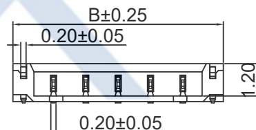
4~5 Pin Without Sticking Point
