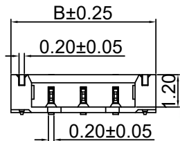
2~3 Pin Without Sticking Point
