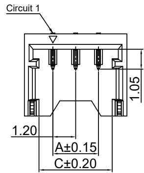
2~3 Pin Without Sticking Point
